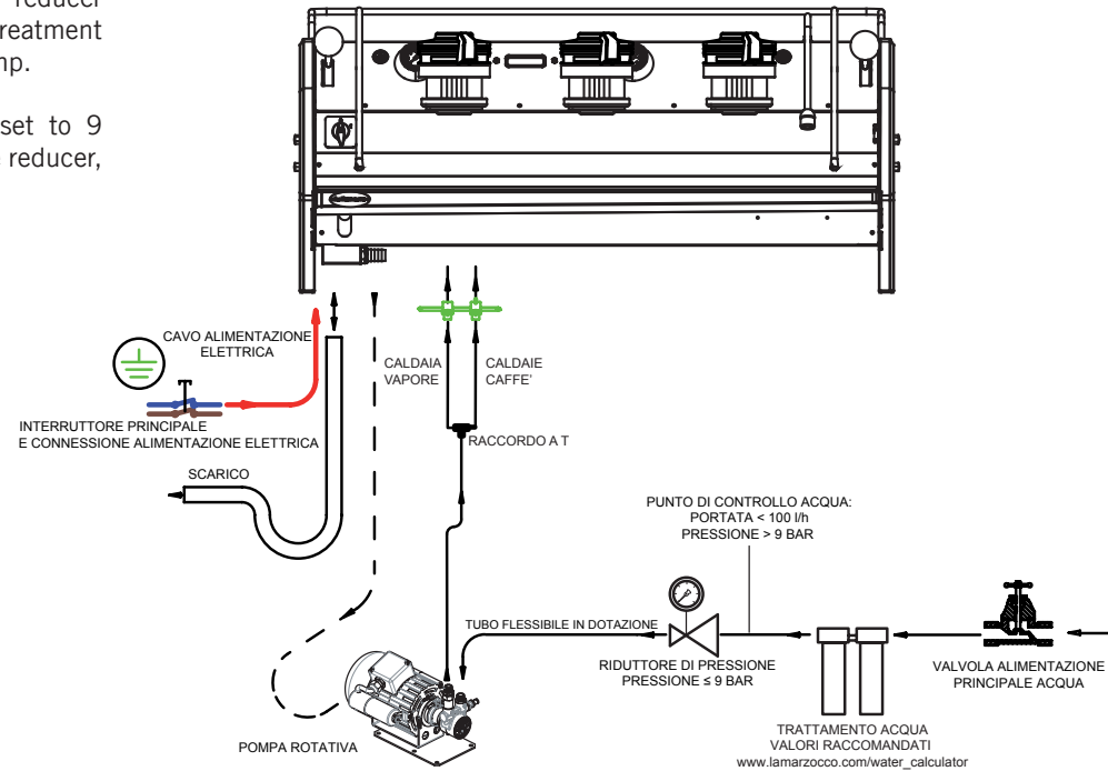
Fig. 4 - Installation guide - type 2
