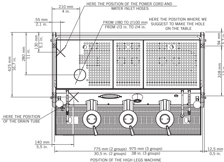
Fig. 2 - Installation guide
